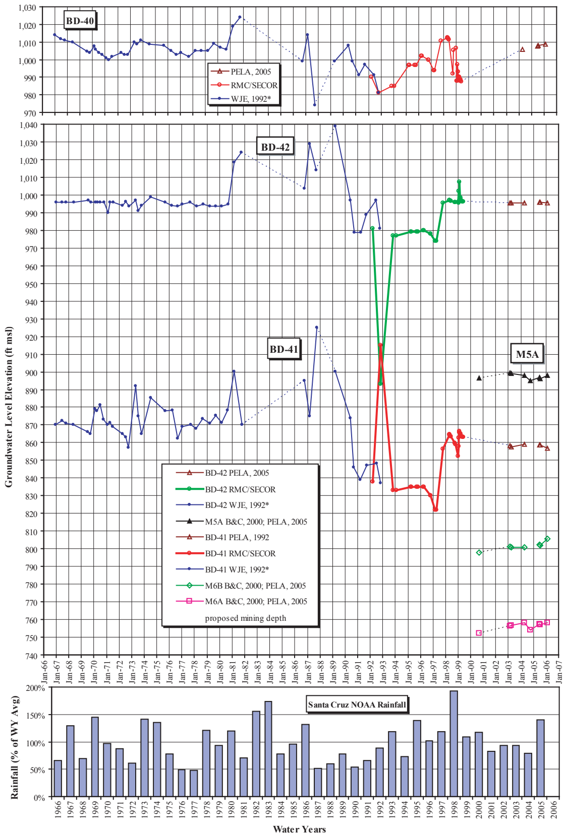
Groundwater Level Hydrographs for Wells BD-40, -41, -42, M5A, M6A, and M6B
